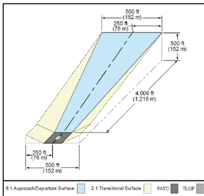
Figure 3C – Vertiport Imaginary Surfaces
