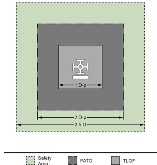
Figure 3B – Relationship and Dimensions
